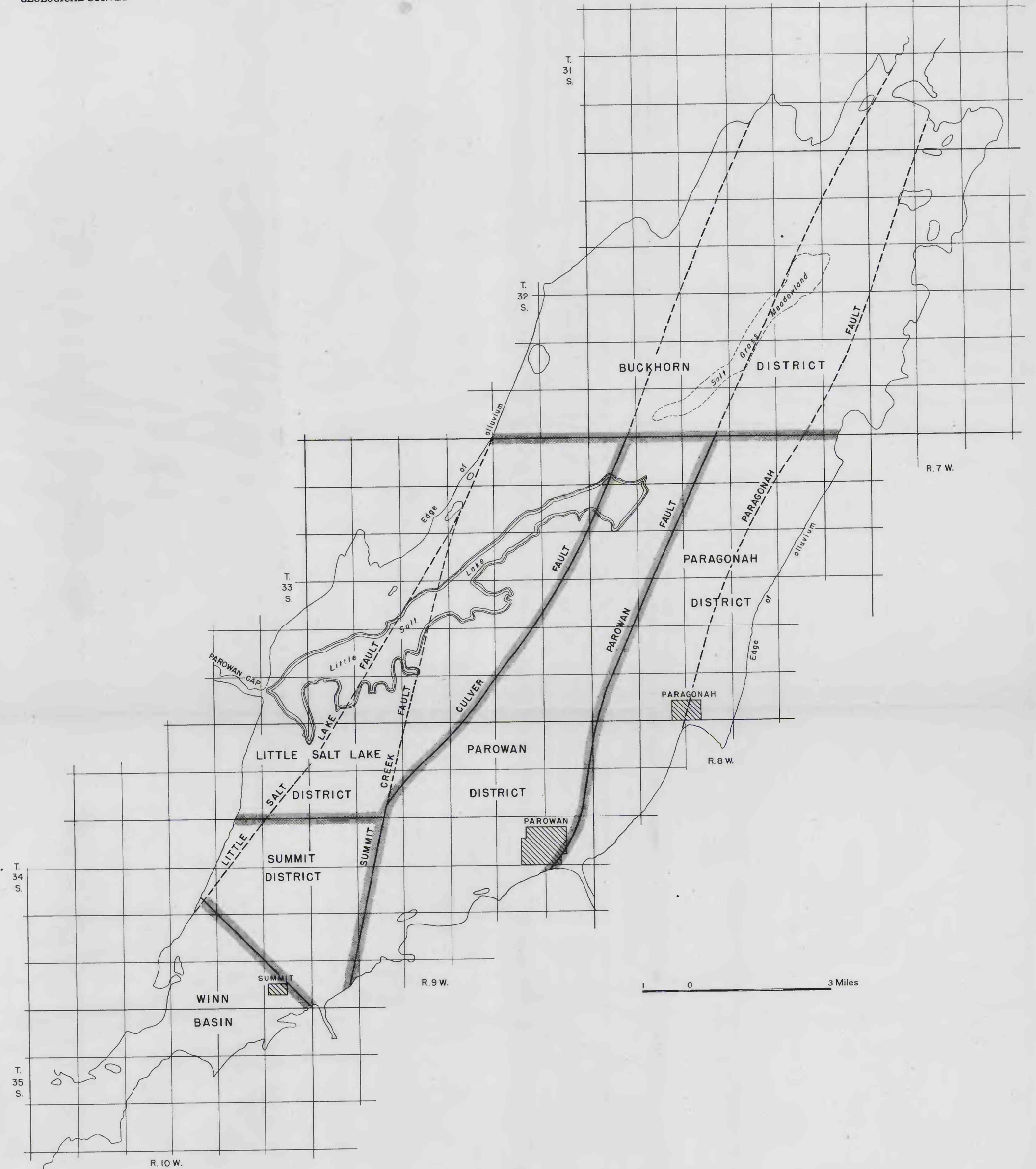
MAP SHOWING GROUND-WATER DISTRICTS IN PAROWAN VALLEY
