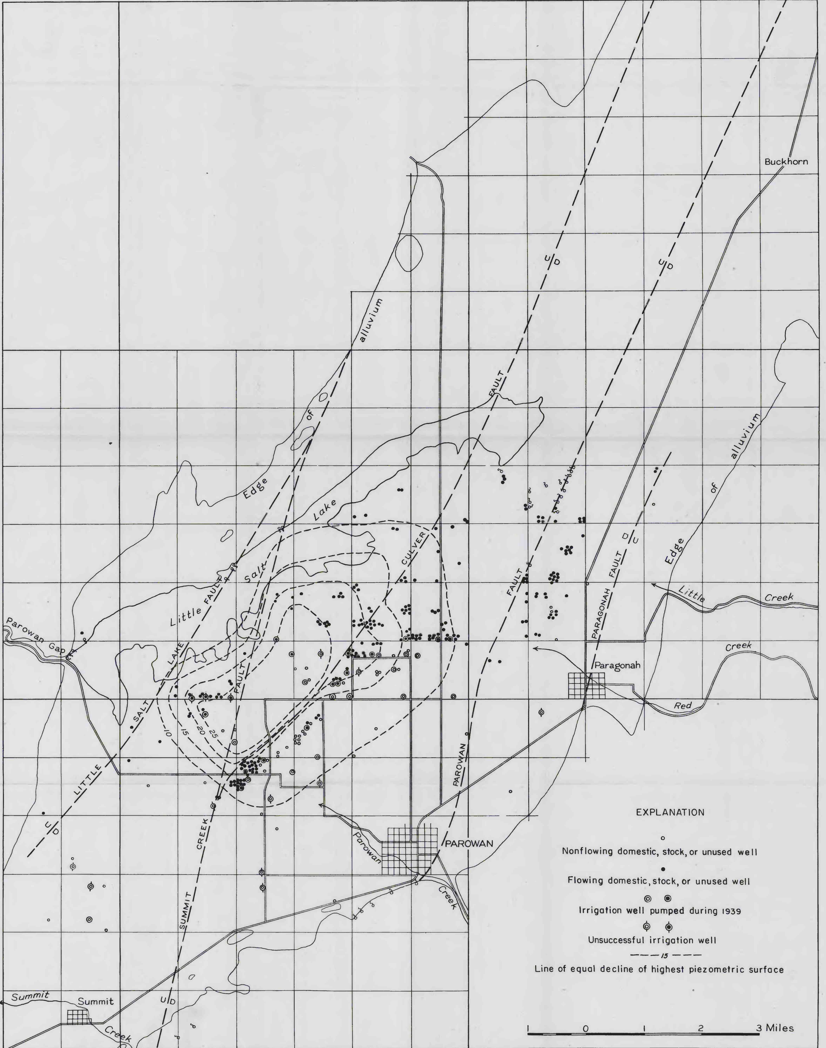
MAP OF PAROWAN VALLEY SHOWING LOCATION OF WELLS AND SPRINGS AND APPROXIMATE DECLINE OF THE HIGHEST PIEZOMETRIC SURFACE BETWEEN ABOUT MARCH 15 AND SEPTEMBER 10, 1940
