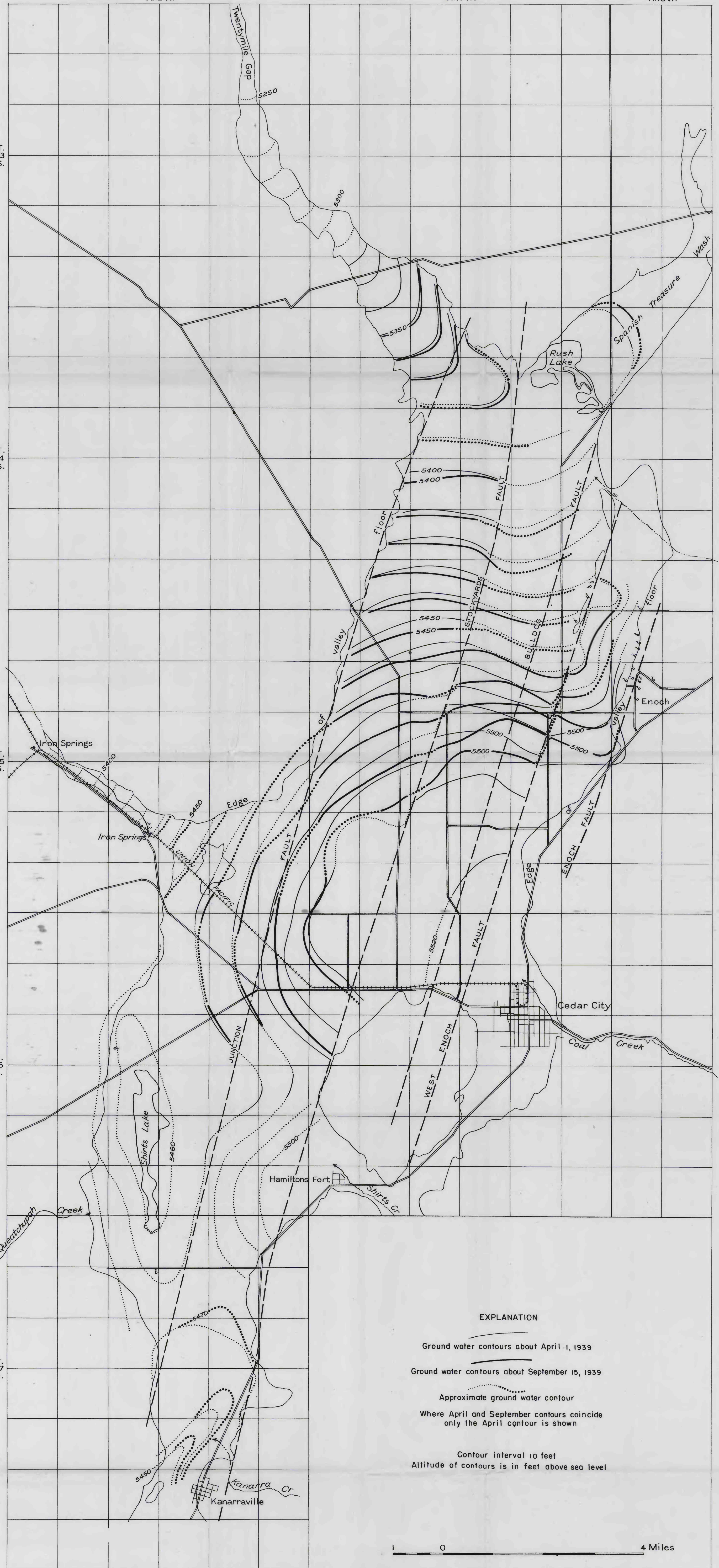
MAP OF CEDAR CITY VALLEY SHOWING GROUND-WATER CONTOURS ABOUT APRIL 1 AND SEPTEMBER 15, 1939
