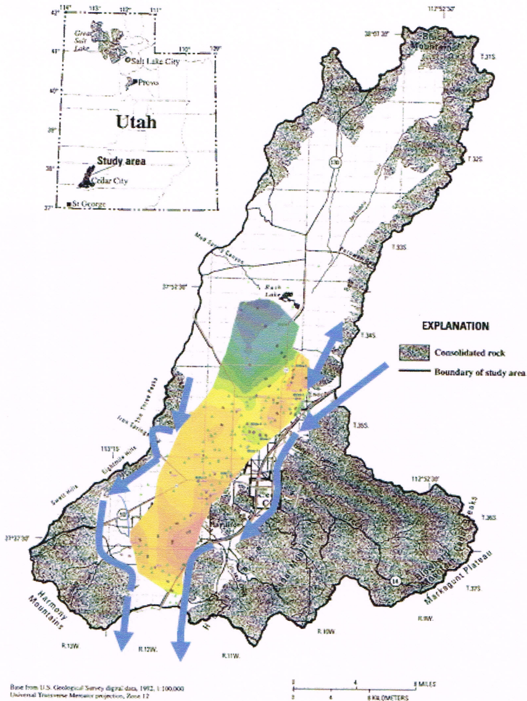
Figure 3. UGS map of land subsidence overlain on map of the Cedar Valley Drainage Basin, with probable water flow along the faults bounding Cedar Valley (not included in USGS model of water flow).
