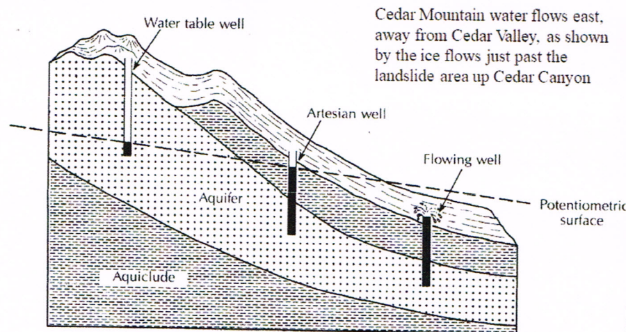
FIGURE 4.21 Artesian and flowing well in confined aquifer.
