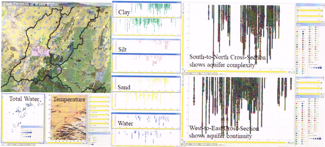
Figure 4. Composite north-south and west-east cross-sections through the Cedar Valley Fill Aquifer.
