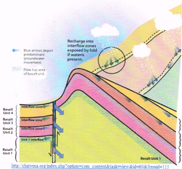
Figure 8. Faults and Dip Force Water Flows from Cedar Mountain to the East and South, so as to not reach the Cedar Valley Fill Aquifer.
