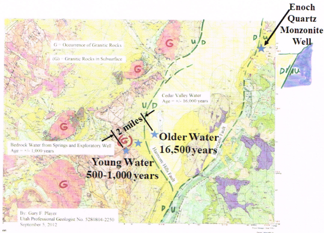
Figure 10. Age Dated Water at Cedar Municipal Wells at Quichapa Springs, Quichapa Creek, and west of Quichapa Lake on the west side of the Cedar Valley Drainage Basin.
