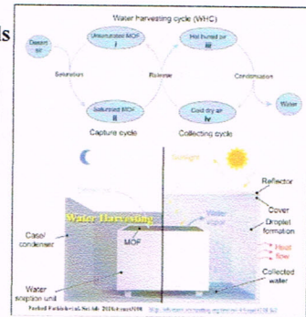
Figure 17. Floating Dew Collectors, Stationary Dew Collectors, Condensation in a Shipping Container, new materials to enhance condensation, and Water Harvesting Machines.
