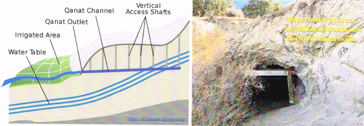
Figure 14. Qanat Technology, developed in ancient Iran about 1,000 B.C. provides another alternative for tapping Bedrock Aquifers outside of the Cedar Valley Fill Aquifer.
