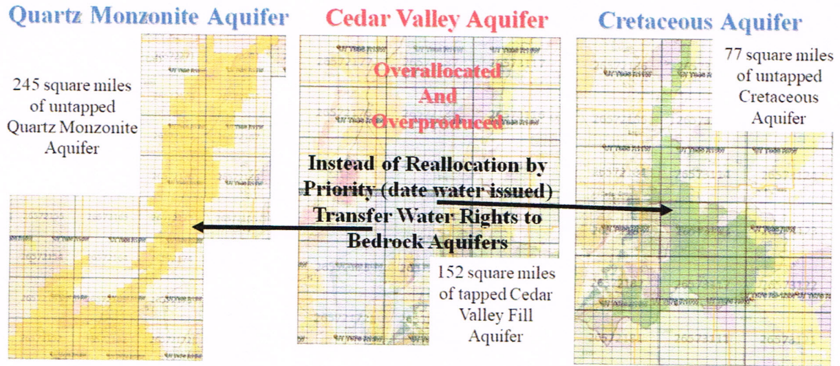
Figure 7. Spatial extent of the untapped Quartz Monzonite Aquifer, the overallocated and over produced Cedar Valley Fill Aquifer, and untapped Cretaceous Aquifer.
