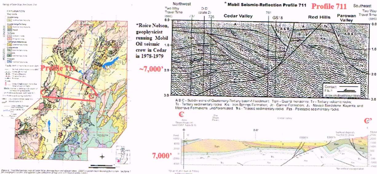
Figure 5. Map, seismic cross-section, and geologic cross-section across the Cedar Valley Fill Aquifer.
